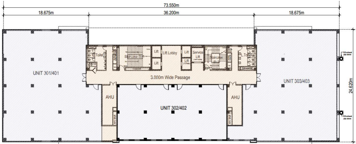
Third & Fourth Floor Plan
